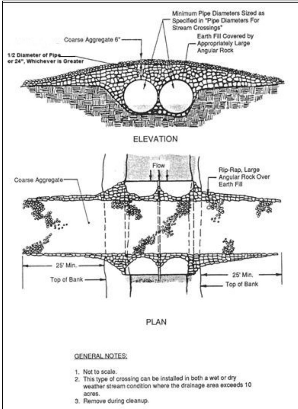
Figure TSC-1 Culvert Stream Crossing
