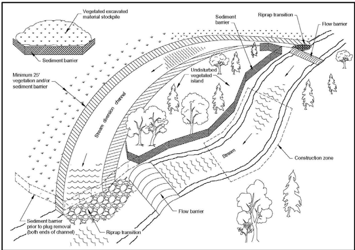
Figure SDC – 1: Typical Stream Diversion Channel Layout.
