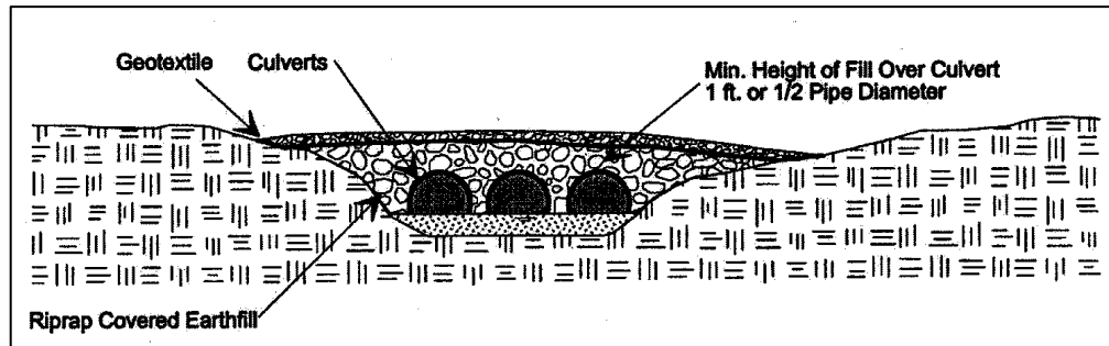
Figure TSC-1 Typical Temporary Culvert Stream Crossing
